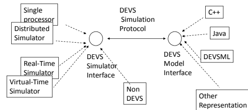
Figure 4: Conceptual Architecture of Standard
