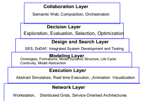
Figure 2 Architecture for Modeling and Simulation
