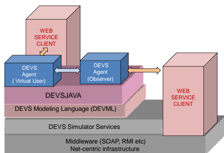
Figure 7 DEVS/SOA interoperability
