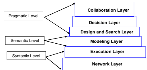
Figure 3 Associating Linguistic Levels with Layers of Modeling and Simulation
