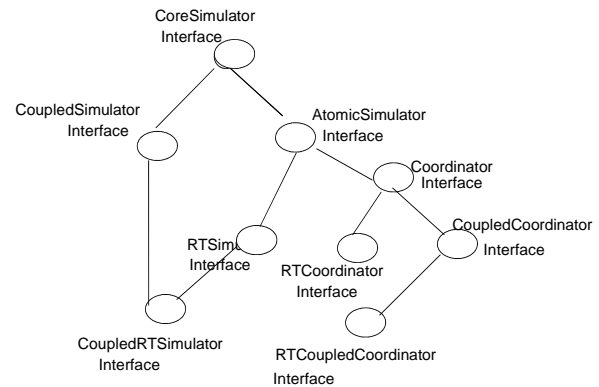
Figure 6 DEVS Simulator Interfaces
